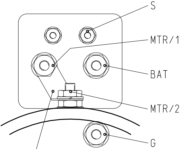
ANLASSER/STARTER A (DELCO REMY)
