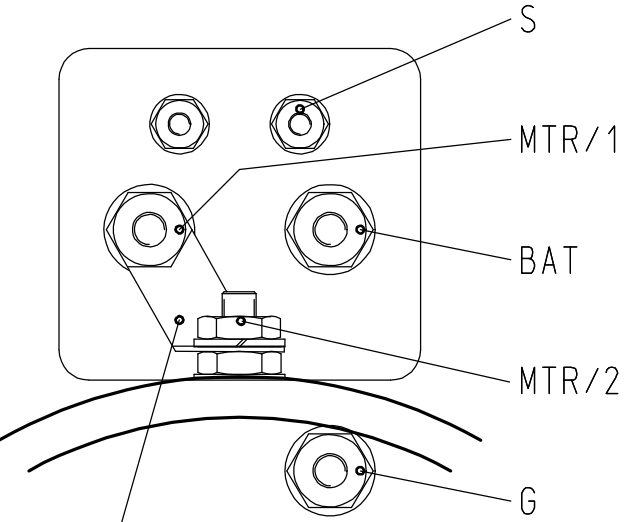
ANLASSER/STARTER B (DELCO REMY)
